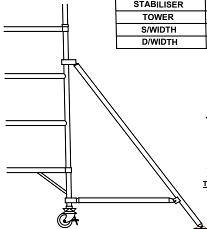
STATIC STABILISER
